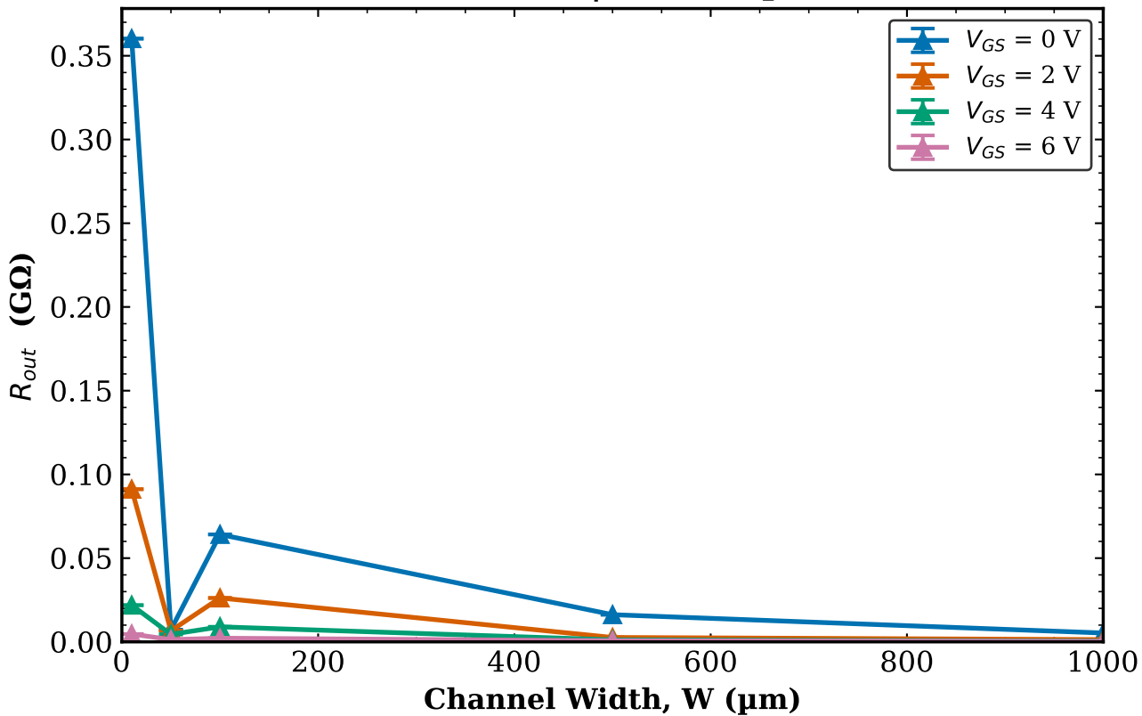
TFT1 Transistor 2 R_{out} vs W | L = 20\text{ }\mu\text{m}
